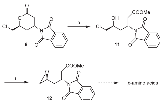
Scheme 3. Synthesis of epoxide 12 . a) cat. HCl, MeOH, \Delta , quant.; b) DBU, \text{CH}_2\text{Cl}_2 , 82%; alternatively: a,b) \text{K}_2\text{CO}_3 , MeOH, 69%.
