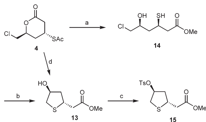
Scheme 4. Synthesis of tosylate 15 . a) cat. HCl, MeOH, quant.; b) DBU, CH 2 Cl 2 , 65%; c) TsCl, NEt 3 , cat. DMAP, CH 2 Cl 2 , 76%; d) K 2 CO 3 , MeOH, 53%.
