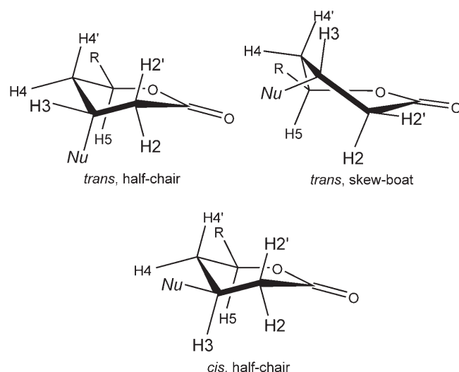
Figure 1. Conformers of 3,5-disubstituted \delta -lactones.
