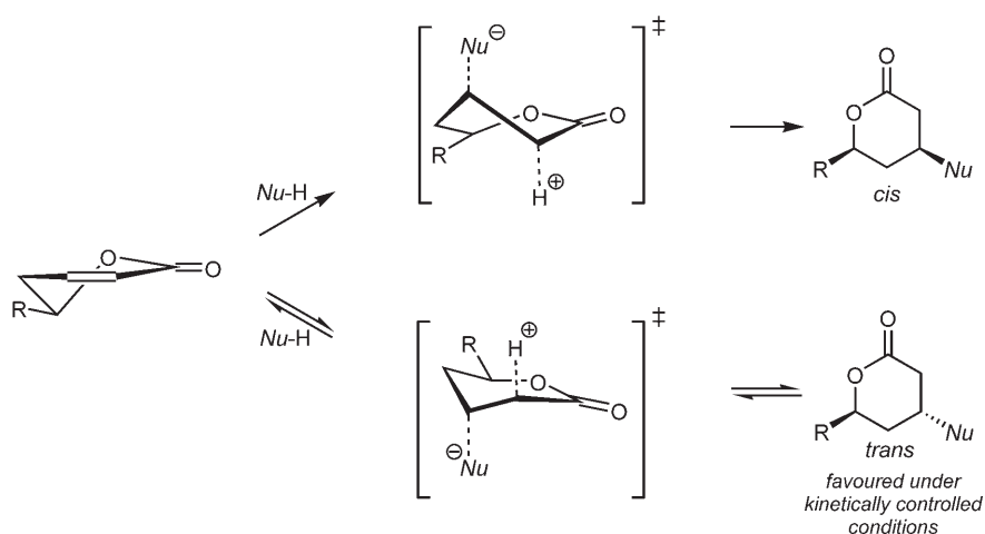
Scheme 2. Stereochemical course of the base-catalysed conjugate addition of nucleophiles Nu-H to \alpha,\beta -unsaturated \delta -lactones. [10]
