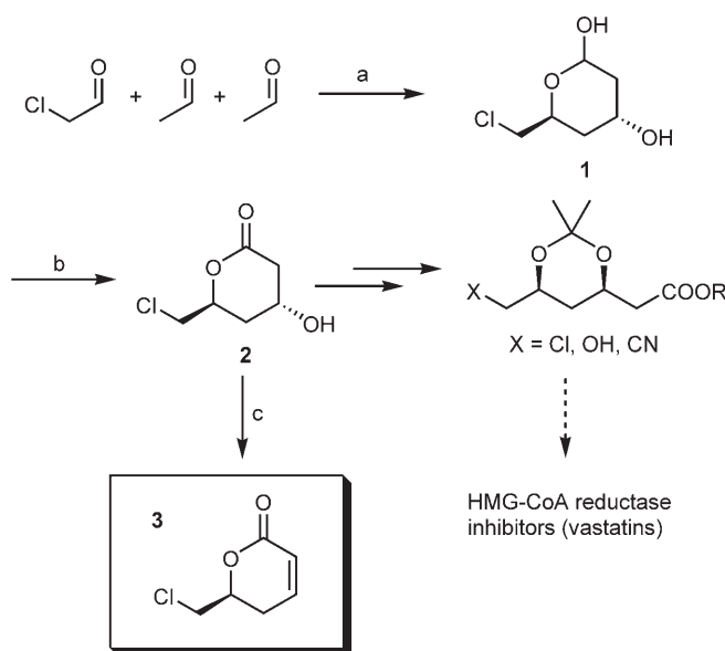
Scheme 1. Chemoenzymatic synthesis of lactone 3 . a) DERA, H 2 O, pH 7 (refs. [2,4a] ); b) Br 2 , H 2 O, pH 5–6 (ref. [4b] ); c) cat. TsOH, toluene, \Delta , 84–87%.
